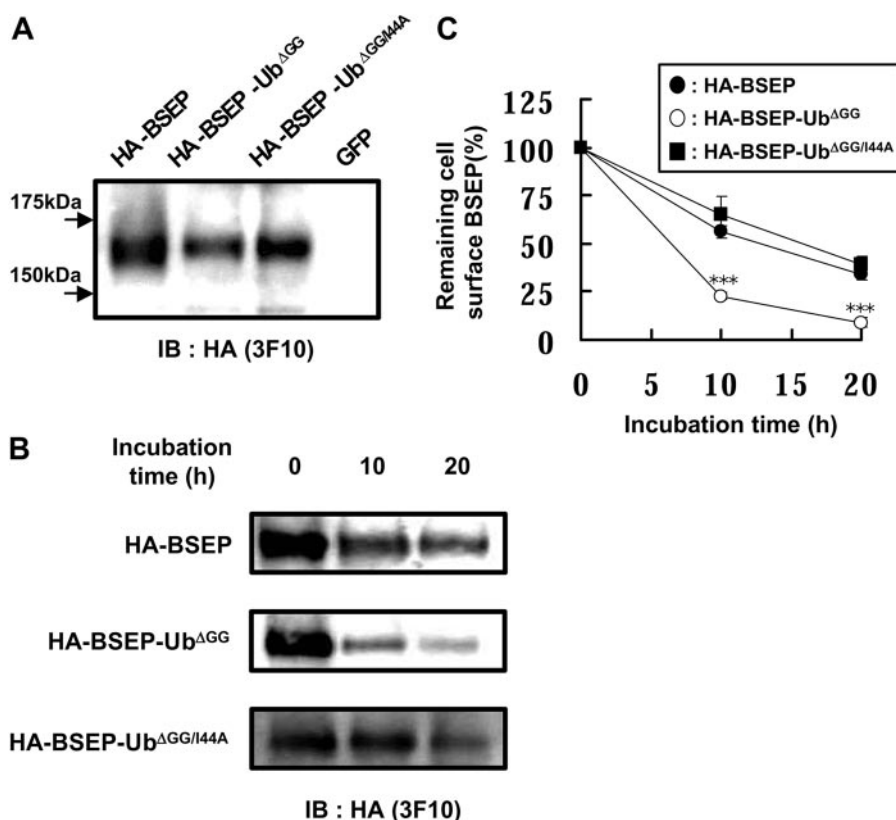
Fig. 4. Determination of the degradation rate of cell-surface-resident BSEP-Ub chimera. A, cell-surface expression of HA-BSEP, HA-BSEP-Ub ΔGG , and HA-BSEP-Ub ΔGG/I44A in MDCK II cells. The cell-surface fractions of MDCK II cells expressing HA-BSEP, HA-BSEP-Ub ΔGG , HA-BSEP-Ub ΔGG/I44A , and GFP were isolated by cell-surface biotinylation as described under Materials and Methods . Prepared specimens were separated by 6% SDS-PAGE and subjected to Western blot analysis. B, the degradation rate of cell-surface-resident HA-BSEP, HA-BSEP-Ub ΔGG , and HA-BSEP-Ub ΔGG/I44A . After cell-surface biotinylation, MDCK II cells expressing HA-BSEP, HA-BSEP-Ub ΔGG , and HA-BSEP-Ub ΔGG/I44A were incubated for the indicated time at 37°C. Remaining biotinylated proteins isolated with streptavidin beads were separated by 6% SDS-PAGE and subjected to Western blot analysis. C, quantification of band density indicating HA-BSEP, HA-BSEP-Ub ΔGG , and HA-BSEP-Ub ΔGG/I44A in A. The intensity of the band indicating HA-BSEP, HA-BSEP-Ub ΔGG , and HA-BSEP-Ub ΔGG/I44A was quantified by Image Gauge software and expressed as respective percentages of the BSEP present at 0 h. ●, ○, and ■ represent remaining cell-surface HA-BSEP, HA-BSEP-Ub ΔGG , and HA-BSEP-Ub ΔGG/I44A , respectively, in MDCK II cells. Each bar represents the mean ± S.E., n = 3 to 5. Asterisks represent statistically significant differences between HA-BSEP and HA-BSEP-Ub ΔGG , ***, P < 0.001.
