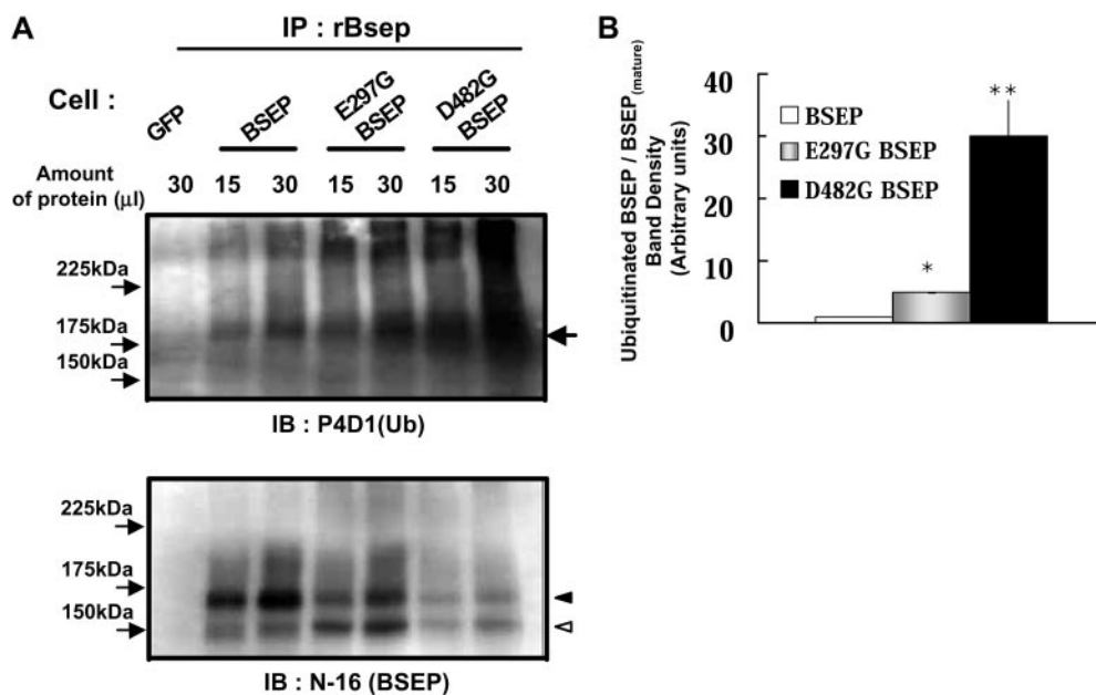
Fig. 2. The effect of PFIC2-type mutations on short-chain ubiquitination of BSEP. A, short-chain ubiquitination susceptibility of PFIC2-type mutated BSEPs, E297G BSEP and D482G BSEP. BSEP and PFIC2-type mutated BSEPs were immunoprecipitated from MDCK II cells expressing BSEP, PFIC2-type mutated BSEPs, and GFP with anti-rBsep antibody. Immunoprecipitates (15 and 30 \mu l) were separated by 6% SDS-PAGE and subjected to Western blot analysis. Arrow, filled and open arrowheads indicate the short-chain ubiquitinated BSEP, the mature and immature forms of BSEP, respectively. B, quantification of the short-chain ubiquitinated BSEP normalized with regard to the mature form of BSEP in A. Data are derived from the intensity of the band indicating the short-chain ubiquitinated BSEP and the mature form of BSEP from 15 \mu l of each specimen applied. Band density was quantified by Image Gauge software. Open, gray, and closed columns represent the ratio of band density indicating the short-chain ubiquitinated BSEP to that indicating the mature form of BSEP in MDCK II cells expressing BSEP, E297G BSEP, and D482G BSEP, respectively. Each bar represents the mean \pm S.E., n = 3 to 4. Asterisks represent statistically significant differences between BSEP and mutated BSEP, *, P < 0.05 , and **, P < 0.01 .
