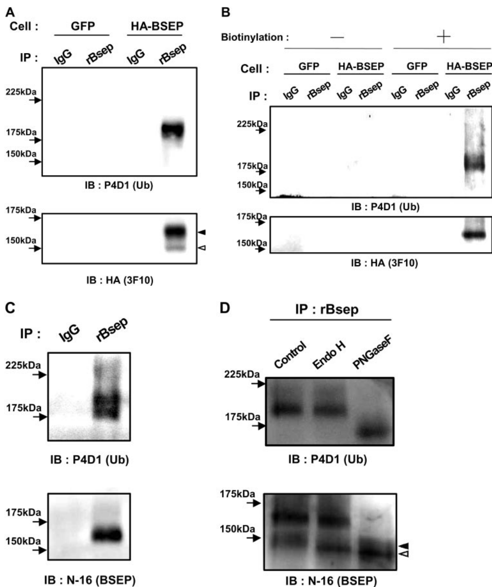
Fig. 1. Ubiquitination of BSEP/Bsep. A , ubiquitination of BSEP in MDCK II cells. BSEP was immunoprecipitated from MDCK II cells expressing HA-BSEP and GFP with anti-rBsep antibody. Immunoprecipitates were separated by 6% SDS-PAGE and subjected to Western blot analysis. Rabbit IgG served as a negative control. Filled and open arrowheads indicate the mature and immature forms of BSEP, respectively. B , ubiquitination of cell-surface-resident BSEP in MDCKII cells. The cell-surface fraction of MDCKII cells expressing HA-BSEP and GFP was labeled with or without biotin and isolated with ImmunoPure StreptAvidin as described under Materials and Methods . Cell-surface-resident BSEP was immunoprecipitated from these specimens with anti-rBsep antibody. Immunoprecipitates were separated by 6% SDS-PAGE and subjected to Western blot analysis. C , ubiquitination of Bsep in rCMVs. Bsep was immunoprecipitated from solubilized rCMVs with anti-rBsep antibody. Immunoprecipitates were separated by 6% SDS-PAGE and subjected to Western blot analysis. D , the extent of glycosylation of ubiquitinated BSEP. Immunoprecipitated specimens from MDCK II cells expressing BSEP with anti-rBsep antibodies were digested by EndoH or PNGaseF. The deglycosylated proteins were separated by 6% SDS-PAGE and subjected to Western blot analysis. Filled and open arrowheads indicate the core- and nonglycosylated form of BSEP, respectively.
