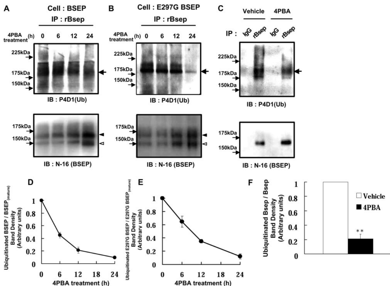
Fig. 3. The effect of 4PBA treatment on short-chain ubiquitination of BSEP/Bsep. A and B, short-chain ubiquitination susceptibility of BSEP (A) and E297G BSEP (B) in 4PBA-treated MDCK II cells. BSEP was immunoprecipitated from MDCK II cells expressing BSEP after 4PBA (1 mM) treatment for the indicated period with anti-rBsep antibody. Immunoprecipitates were separated by 6% SDS-PAGE and subjected to Western blot analysis. Arrows, filled arrowheads, and open arrowheads indicate the short-chain ubiquitinated BSEP and the mature and immature forms of BSEP, respectively. C, short-chain ubiquitination susceptibility of Bsep in 4PBA-treated SD rats. Male SD rats (6–7 weeks old) were given 4PBA or vehicle by gavage for 10 days at 0.6 g/kg/day before the experiments. Bsep was immunoprecipitated from solubilized rCMVs prepared from 4PBA-treated SD rats with anti-rBsep antibody. Immunoprecipitates were separated by 6% SDS-PAGE and subjected to Western blot analysis. D and E, quantification of the short-chain ubiquitinated BSEP and E297G BSEP normalized with regard to the mature form of BSEP and E297G BSEP in A and B. Data are derived from the band density indicating the short-chain ubiquitinated BSEP and mature form of BSEP by Image Gauge software. Each bar represents the mean \pm S.E., n = 3 . F, quantification of the short-chain ubiquitinated Bsep normalized with regard to Bsep in C. Data are derived from the intensity of the band indicating the short-chain ubiquitinated Bsep and Bsep by Image Gauge software. Closed and open columns represent the ratio of band density indicating the short-chain ubiquitinated Bsep to Bsep in rCMVs prepared from SD rats, with and without 4PBA, respectively. Each bar represents the mean \pm S.E., n = 4 . Asterisks represent statistically significant differences between vehicle-treated SD rats and 4PBA-treated SD rats, **, P < 0.01 .
